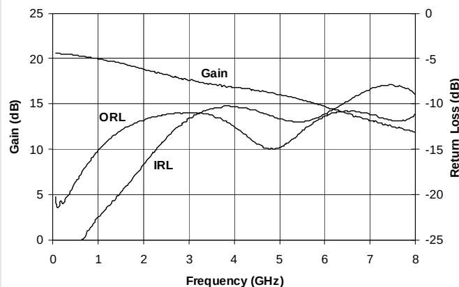
Gain Return Loss versus Frequency, I_D = 80\text{mA} (Typ), Tuned Application Circuit
