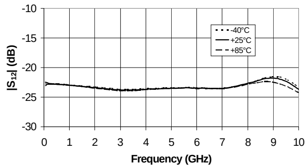
S_{12} vs. Frequency
