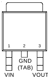
TO-252
