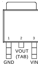
TO-252 (F-Type)
