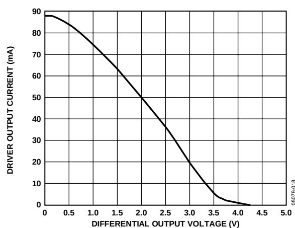
Figure 18. Driver Output Current vs. Differential Output Voltage
