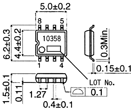
BA10358F(SOP8) (Unit:[mm])
