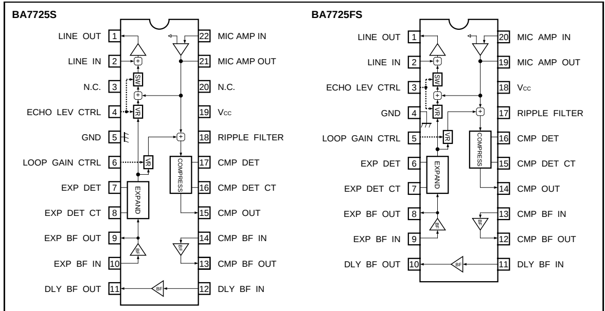
●Block diagram
