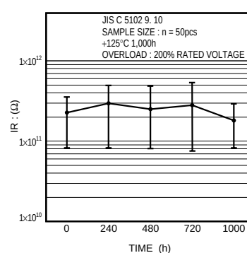
Fig.21 Insulation resistance
