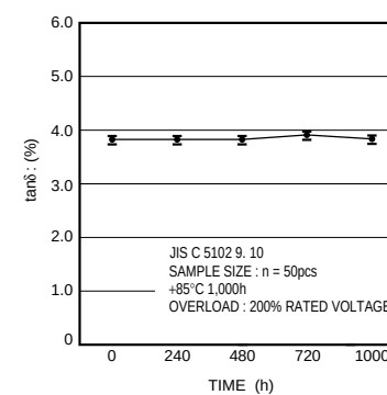
Fig.23 \tan\delta
