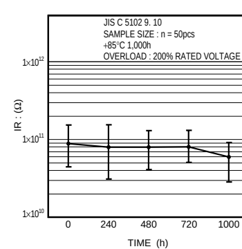
Fig.24 Insulation resistance
