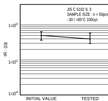
Fig.15 Insulation resistance
