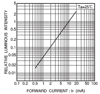
Fig.11 Luminous intensity vs. forward current
