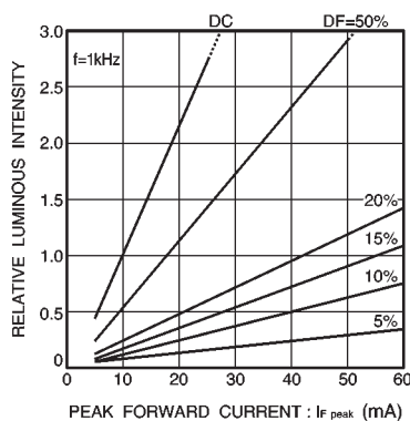
Fig. 25 Luminous intensity vs. peak forward current
