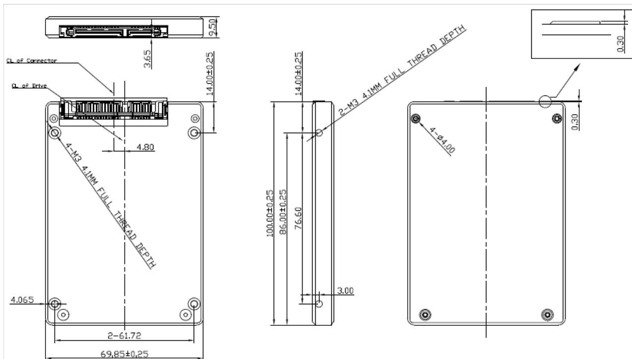
Figure 2-1. Physical dimension
