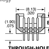
THROUGH-HOLE
