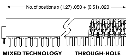
MIXED TECHNOLOGY
