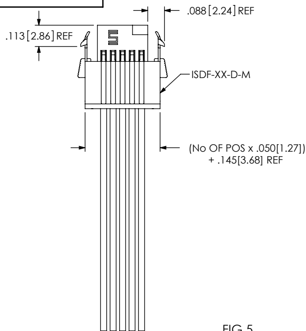
FIG 5 -SR: SINGLE END WITH RETENTION LATCH SFSDX-10-28-XX-XX.XX-SR SHOWN (ONLY AVAILABLE ON -02 THRU -50 POS) (SAME AS FIG 1, UNLESS OTHERWISE STATED)
