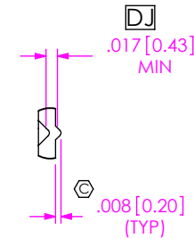
CRIMP DETAIL SCALE: 4:1 (TYP ALL CRIMPS)
