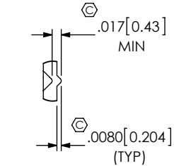
CRIMP DETAIL SCALE: 4:1 (TYP ALL CRIMPS)
