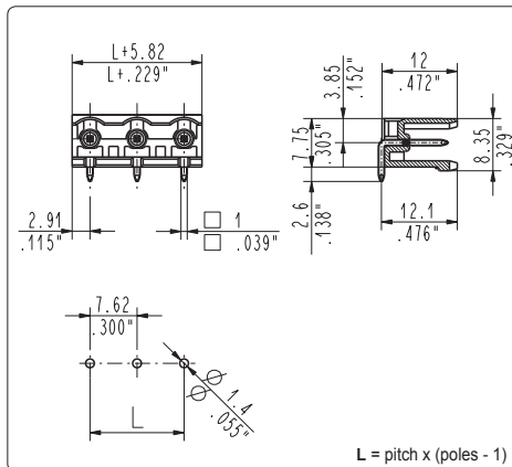
CIM_5A7 270°, side stackable male
