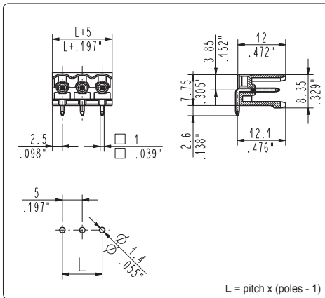
CIM_5A1 270°, side stackable male
