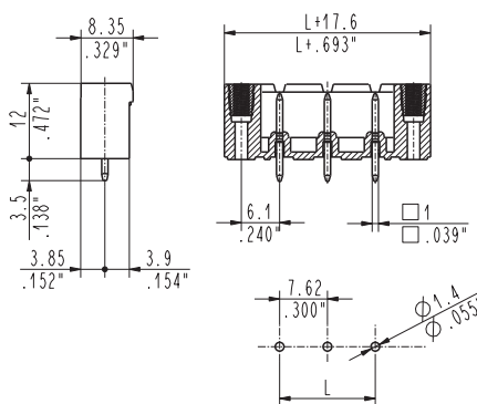
CIM_OV7 straight, locking screw flanges male
