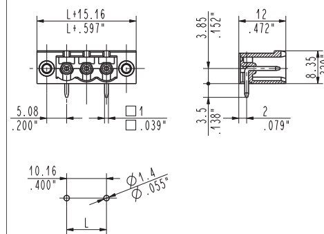
CIM_9V6 90°, locking screw flanges male
