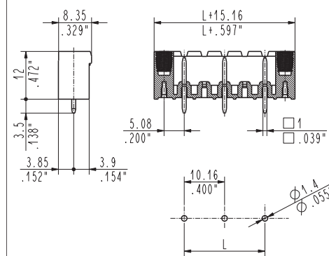
CIM_OV6 straight, locking screw flanges male
