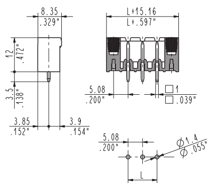
CIM_OV5 straight, locking screw flanges male
