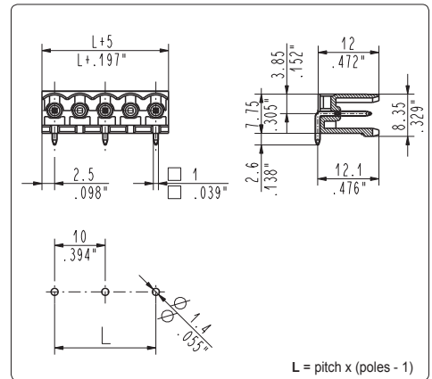
CIM_5A2 270°, side stackable male
