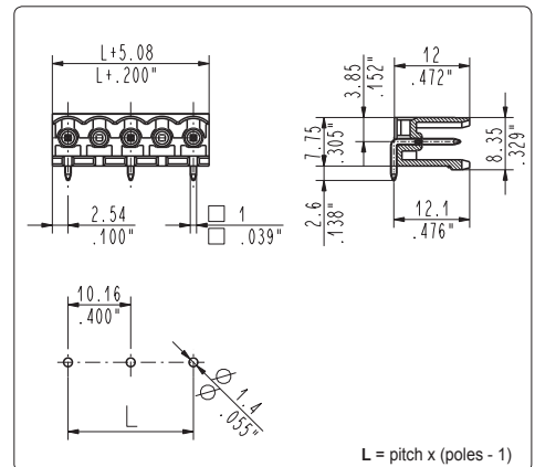
CIM_5A6 270°, side stackable male
