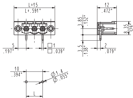
CIM_9V2 90°, locking screw flanges male
