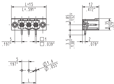
CIM_9V1 90°, locking screw flanges male
