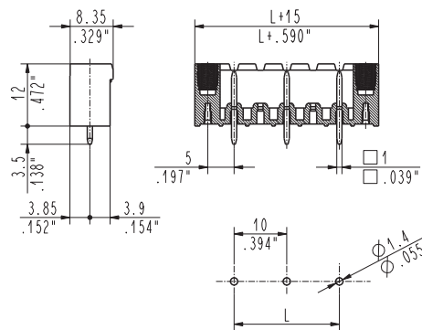
CIM_OV2 straight, locking screw flanges male
