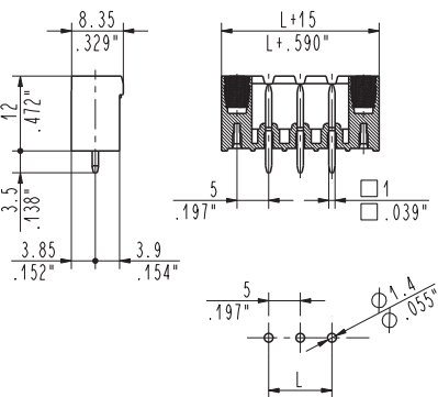
CIM_OV1 straight, locking screw flanges male
