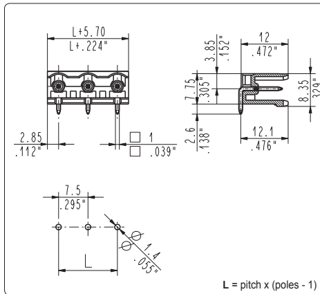
CIM_5A3 270°, side stackable male
