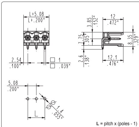
CIM_5A5 270°, side stackable male
