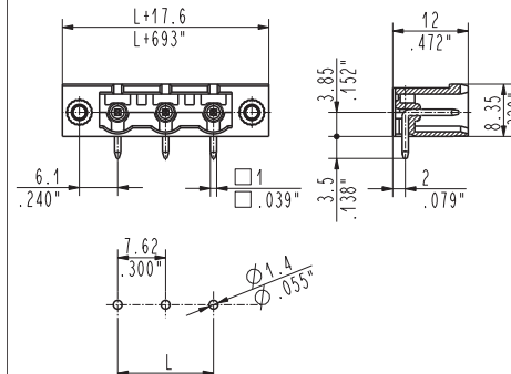
CIM_9V7 90°, locking screw flanges male
