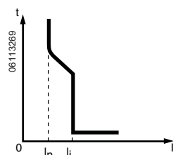
H-Frame Trip Curve
