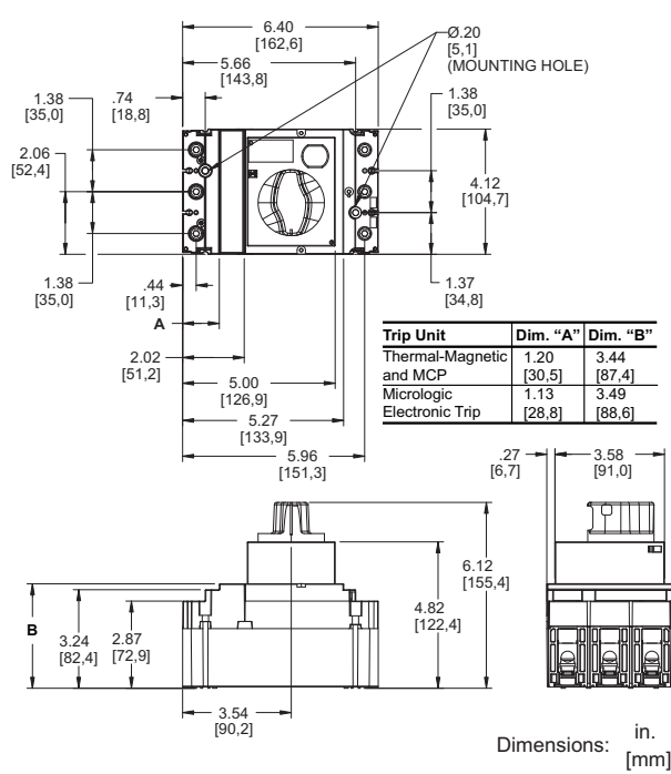
Figure 14: Rotary Handle Detail (PowerPact H-Frame Circuit Breaker)
