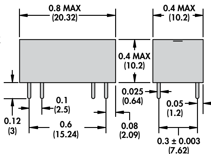
172DIP DPDT
