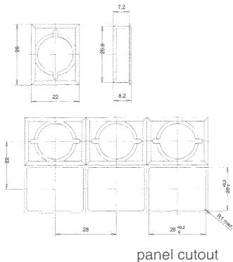
panel cutout
