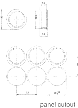
panel cutout
