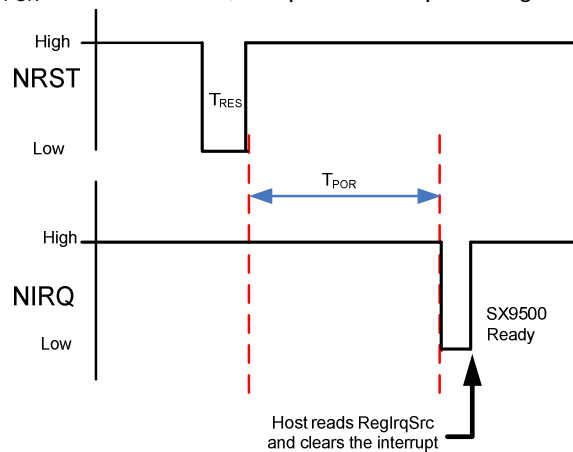
Figure 25: Hardware Reset
