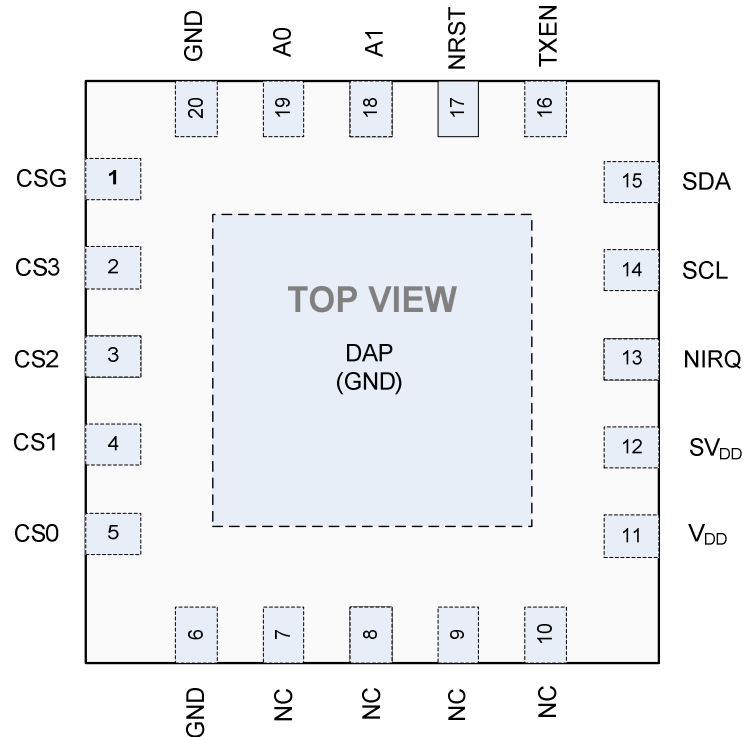
Figure 1: Pin Diagram
