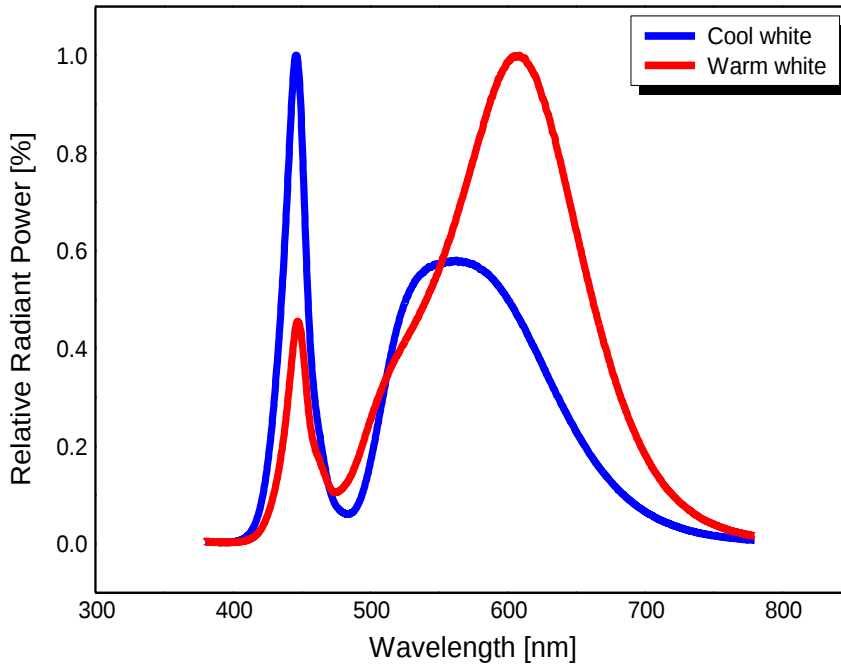
Fig 1. Color Spectrum, Ta = 25℃, IF = 180mA, RH30%
