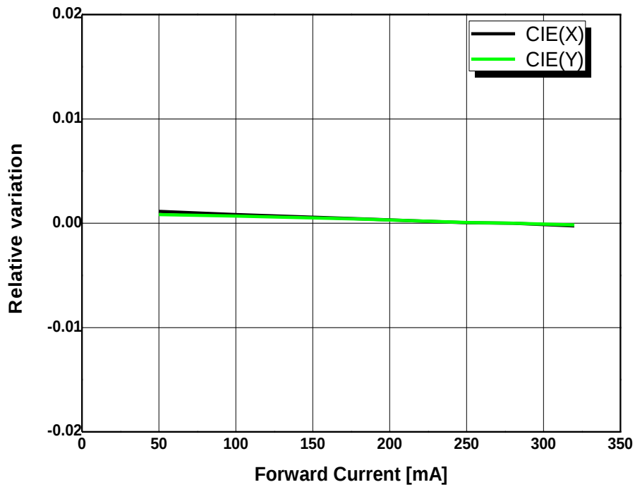
Fig 5. Forward Current vs. CIE X, Y Shift , Ta=25℃ (Warm white)
