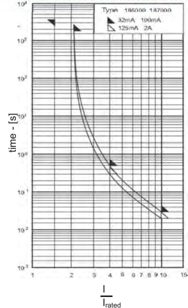
Time-Current Characteristics
