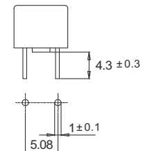
Dimensions [mm]
