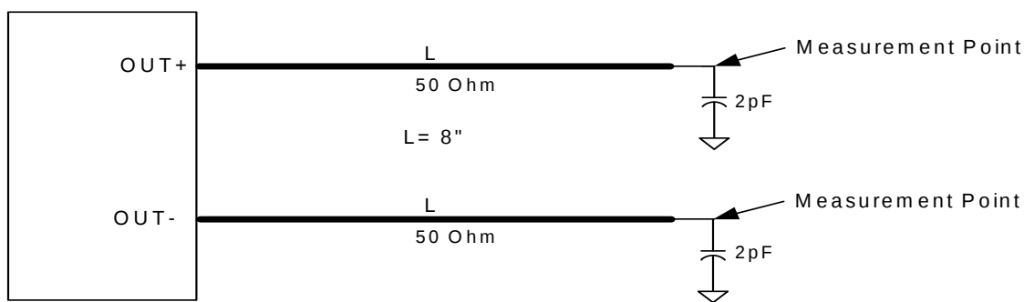
Figure 17. 0.7V Differential Load Configuration
