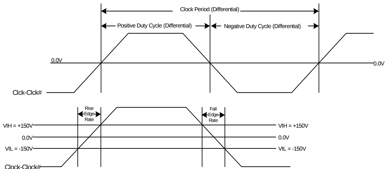
Figure 18. Differential Measurement for Differential Output Signals (for AC Parameters Measurement)
