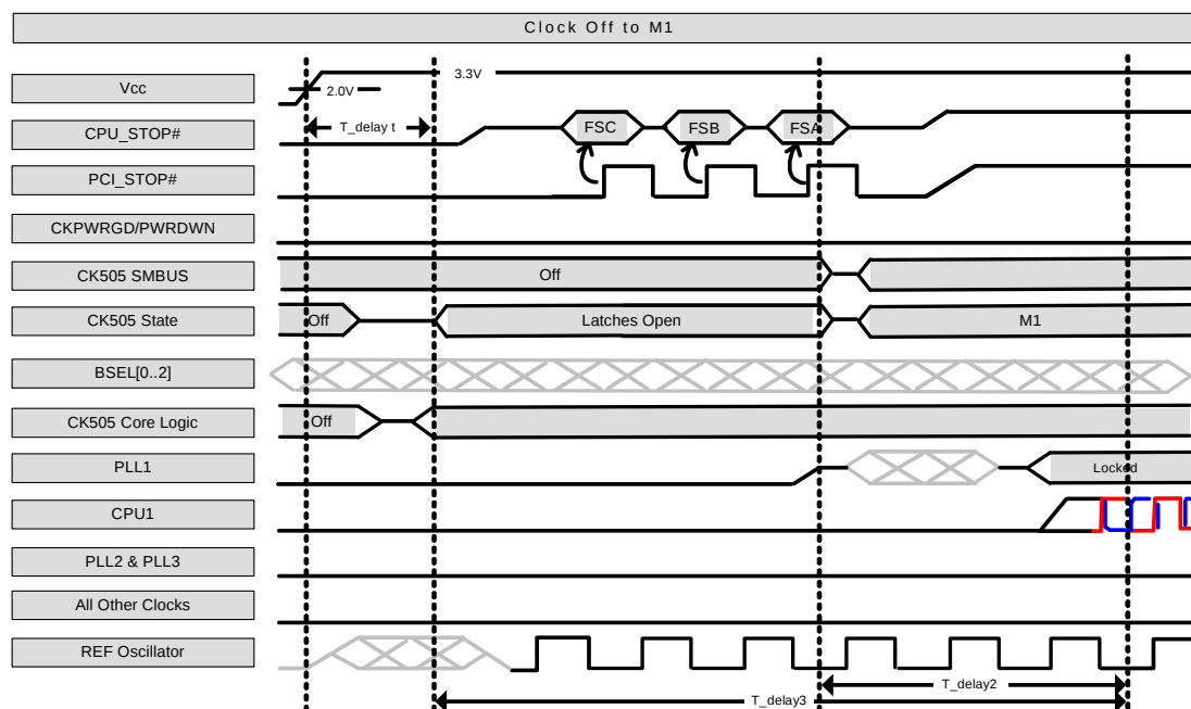
Figure 13. BSEL Serial Latching
