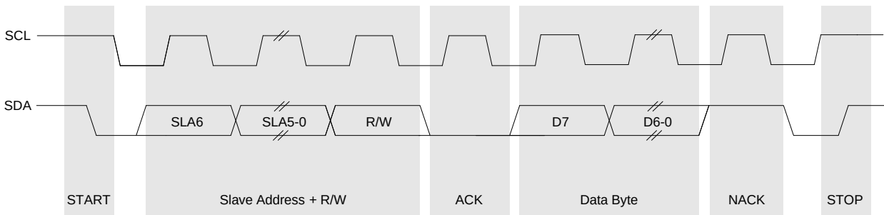
Figure 5. I 2 C Bit Timing Diagram
