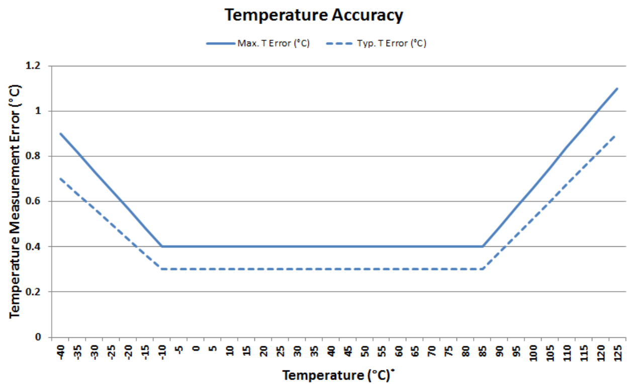
Figure 3. Temperature Accuracy*
