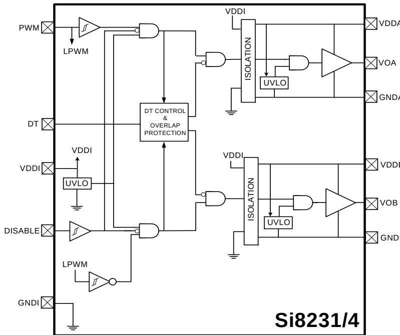
Figure 2. Si8231/4 Single-Input High-Side/Low-Side Isolated Drivers
