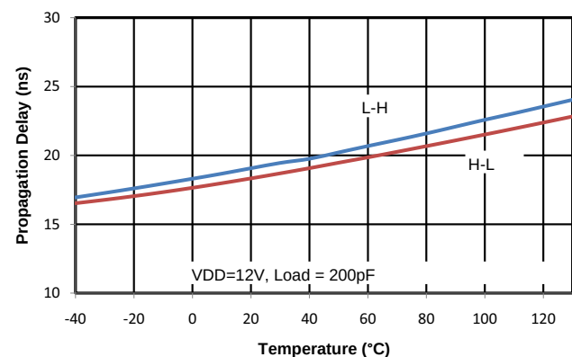
Figure 18. Propagation Delay vs. Temperature
