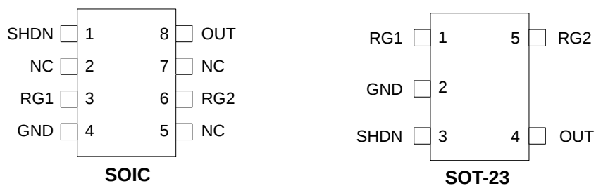
Figure 11. Pin Configuration
