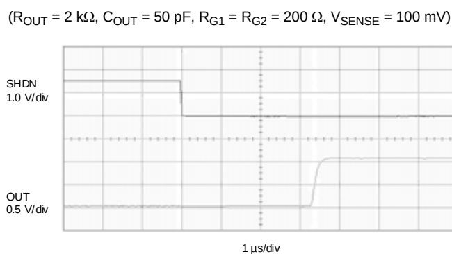
Figure 7. Startup Delay
