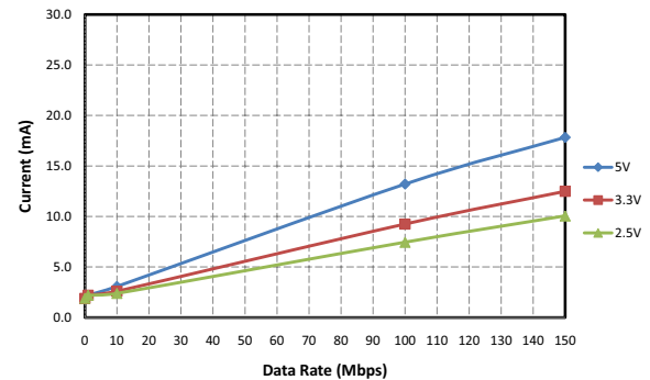
Figure 13. Si8630/35 Typical V_{DD2} Supply Current vs. Data Rate 5, 3.3, and 2.5 V Operation (15 pF Load)
