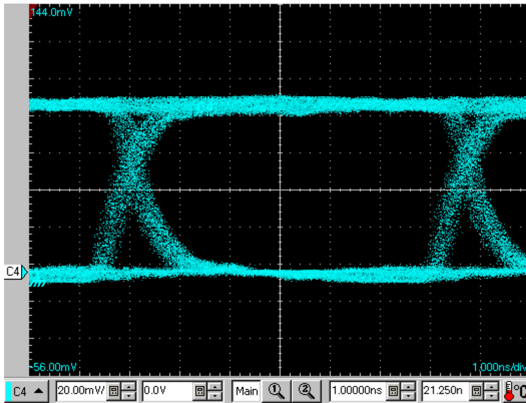
Figure 8. Eye Diagram
