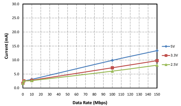
Figure 14. Si8631 Typical V_{DD2} Supply Current vs. Data Rate 5, 3.3, and 2.5 V Operation (15 pF Load)
