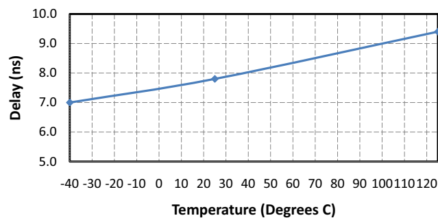
Figure 12. Propagation Delay vs. Temperature
