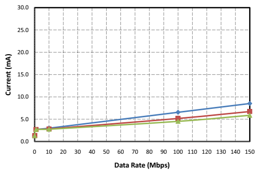
Figure 11. Si8631 Typical V_{DD1} Supply Current vs. Data Rate 5, 3.3, and 2.5 V Operation
