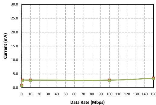
Figure 10. Si8630/35 Typical V_{DD1} Supply Current vs. Data Rate 5, 3.3, and 2.5 V Operation
