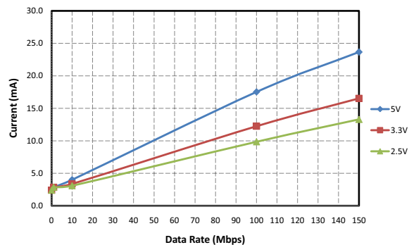
Figure 13. Si8640/45 Typical V_{DD2} Supply Current vs. Data Rate 5, 3.3, and 2.5 V Operation
