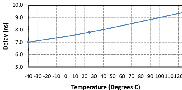
Figure 15. Propagation Delay vs. Temperature
