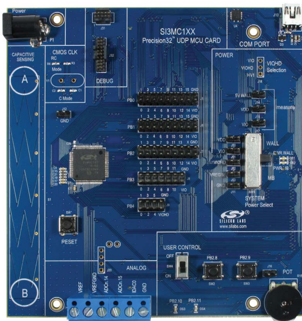
Figure 5. UDP SiM3C1xx MCU Card
