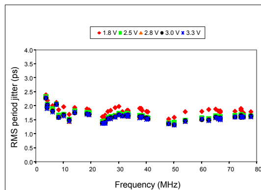
Figure 8. RMS Period Jitter vs Frequency
