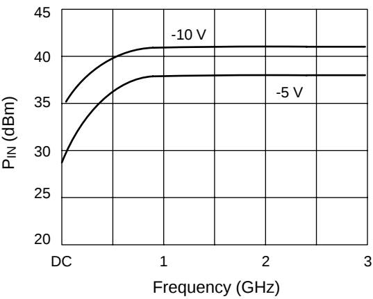
P 1N at 1 dB Compression vs. Frequency and Control Voltage
