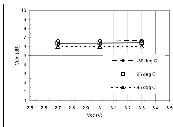
Figure 12. Cell CDMA LNA Gain (Mid Gain) at 881 MHz
