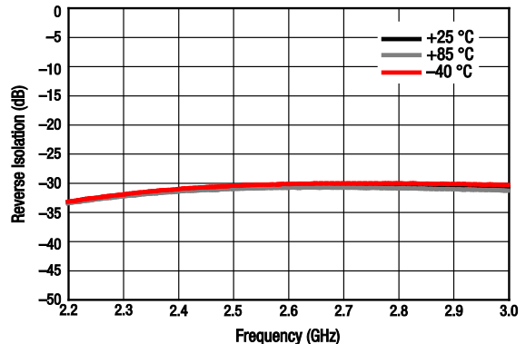
Figure 8. Narrowband Reverse Isolation vs Frequency Over Temperature
