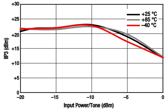
Figure 12. IIP3 vs Input Power Over Temperature @ 2200 MHz ( P_{IN} = -20 dBm, Tone Spacing = 1 MHz)
