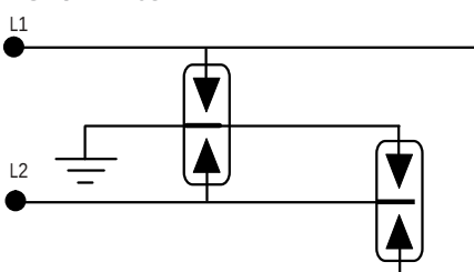
Parallel protection
