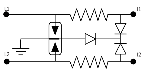
Series protection
