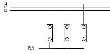
TNC networks
