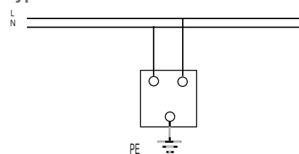
TT - TNS networks (2-pole models)
