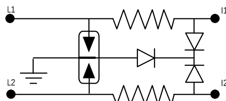
Series protection
