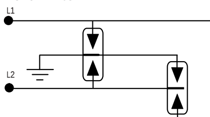
Parallel protection
