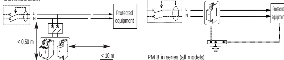
PM Bi (all models) and PM 8 in parallel (all models)
