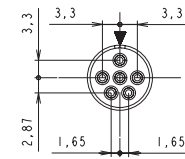
10-98 6 contacts 6 x Ø1.0 (#20)
