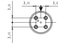
12-4 3 contacts + ground 4 x Ø1.6 (#16)
