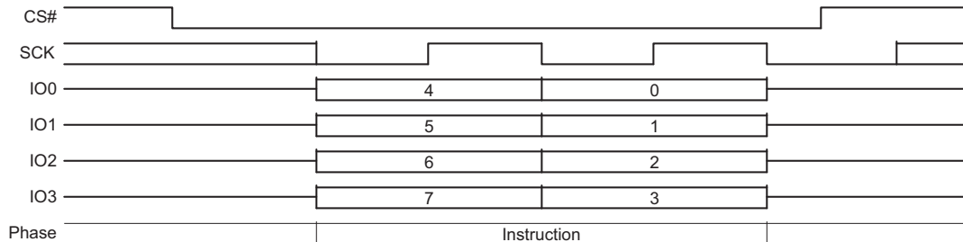
Figure 10.77 DPD Command Sequence QPI Mode
