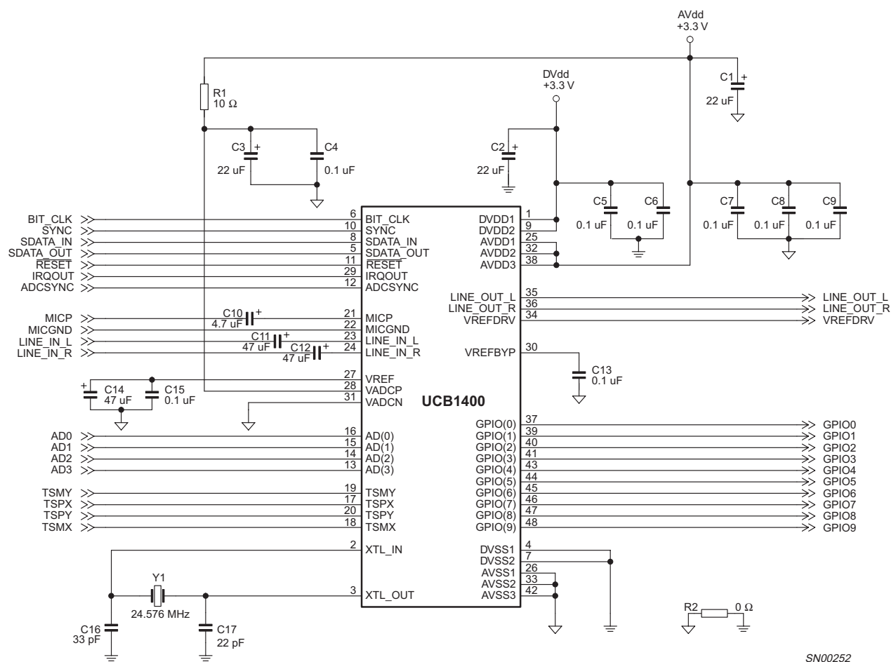
Fig 31. Typical application circuit.
