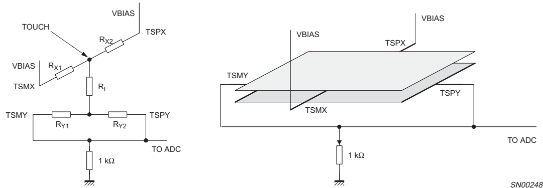
Fig 19. Touch screen setup for pressure-1 measurement (see Table 9).
