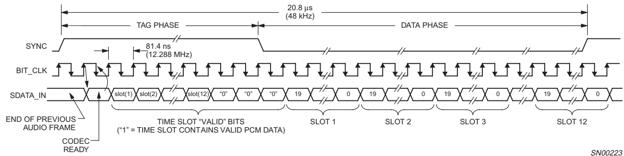
Fig 8. AC-link audio input frame.
