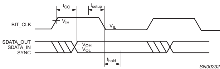
Fig 27. Data output and input timing.
