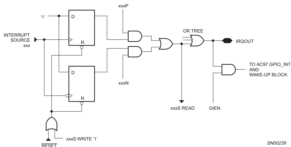
Fig 13. Block diagram of the interrupt controller.
