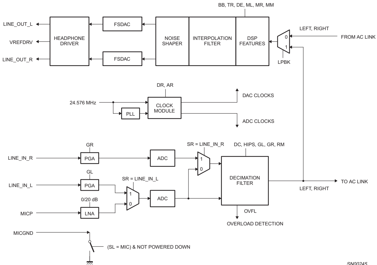
Fig 14. Audio codec block diagram.
