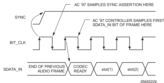
Fig 9. Start of an audio input frame.
