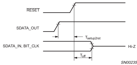
Fig 30. ATE test mode timing.
