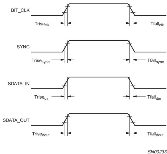
Fig 28. Data rise and fall timing.
