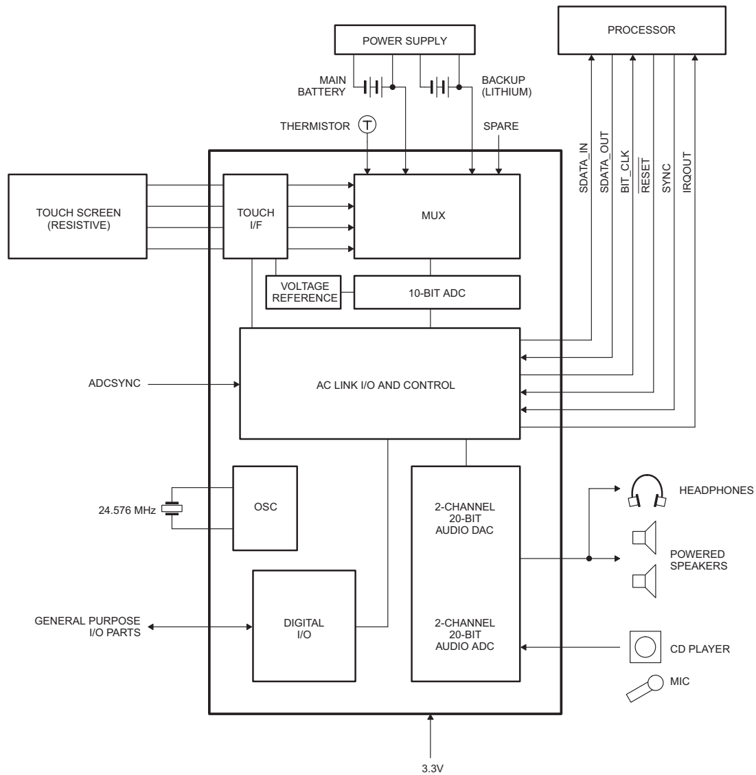
Fig 32. Application block diagram.
