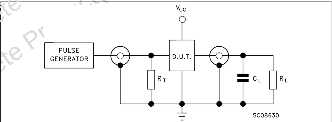
Figure 1. Test circuit
