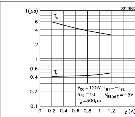
Figure 13. Resistive load switching off times ( h_{FE} = 10 )
