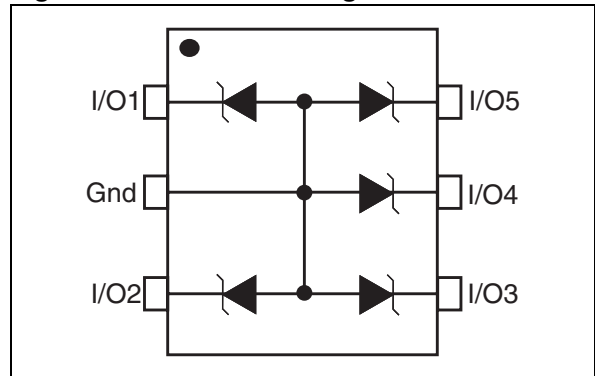
Figure 1. Functional diagram
