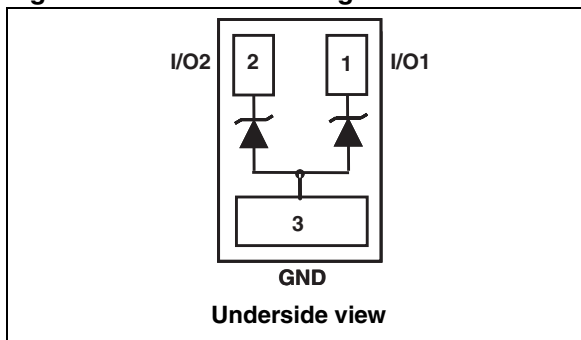
Figure 1. Functional diagram
