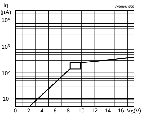
Figure 5. Quiescent current vs. supply voltage
