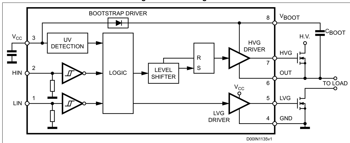
Figure 1. Block diagram
