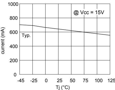
Figure 9. Output sink current vs. temperature
