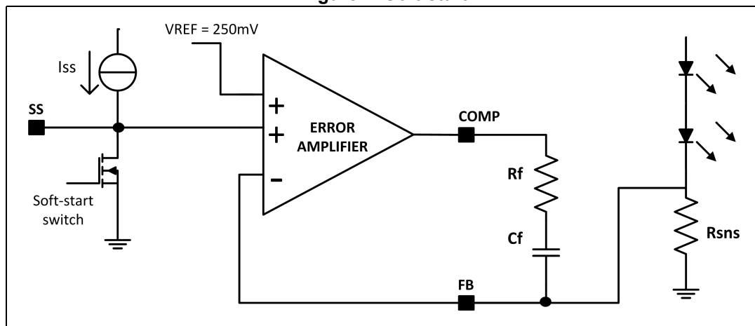
Figure 7. Soft-start
