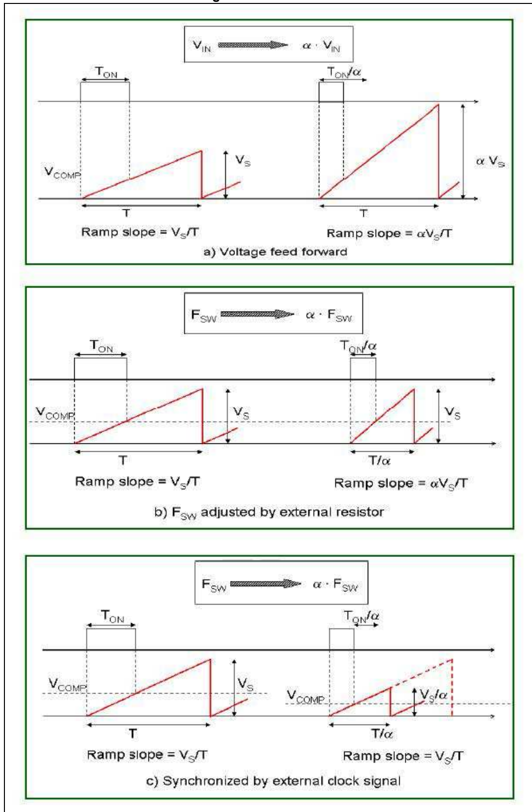
Figure 6. Feedforward
