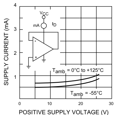
Figure 14. Supply current
