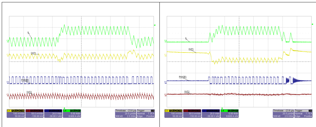
Figure 39. Load transient 0-5 A 2 A/ \mu s OUT1 = 1.5 V SKIP mode
