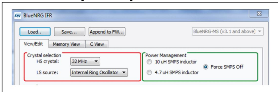
Figure 2: IFR configuration for SPBTLE-RF0
