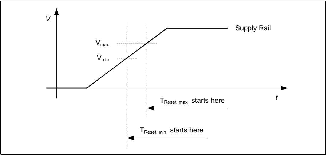
Figure 19. Reset sequence start for Destructive Resets
