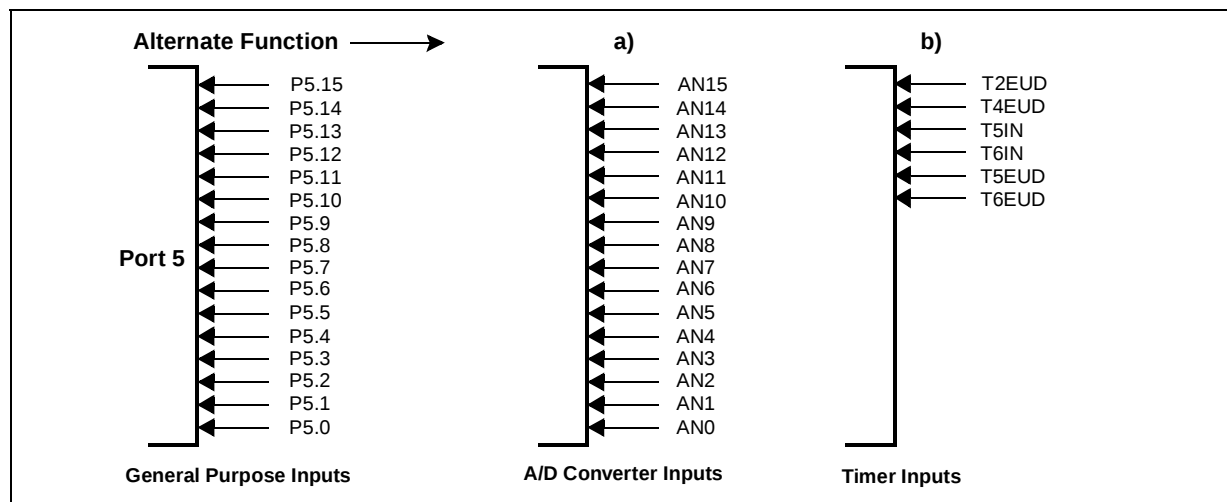
Figure 34 : Port 5 I/O and Alternate Functions
